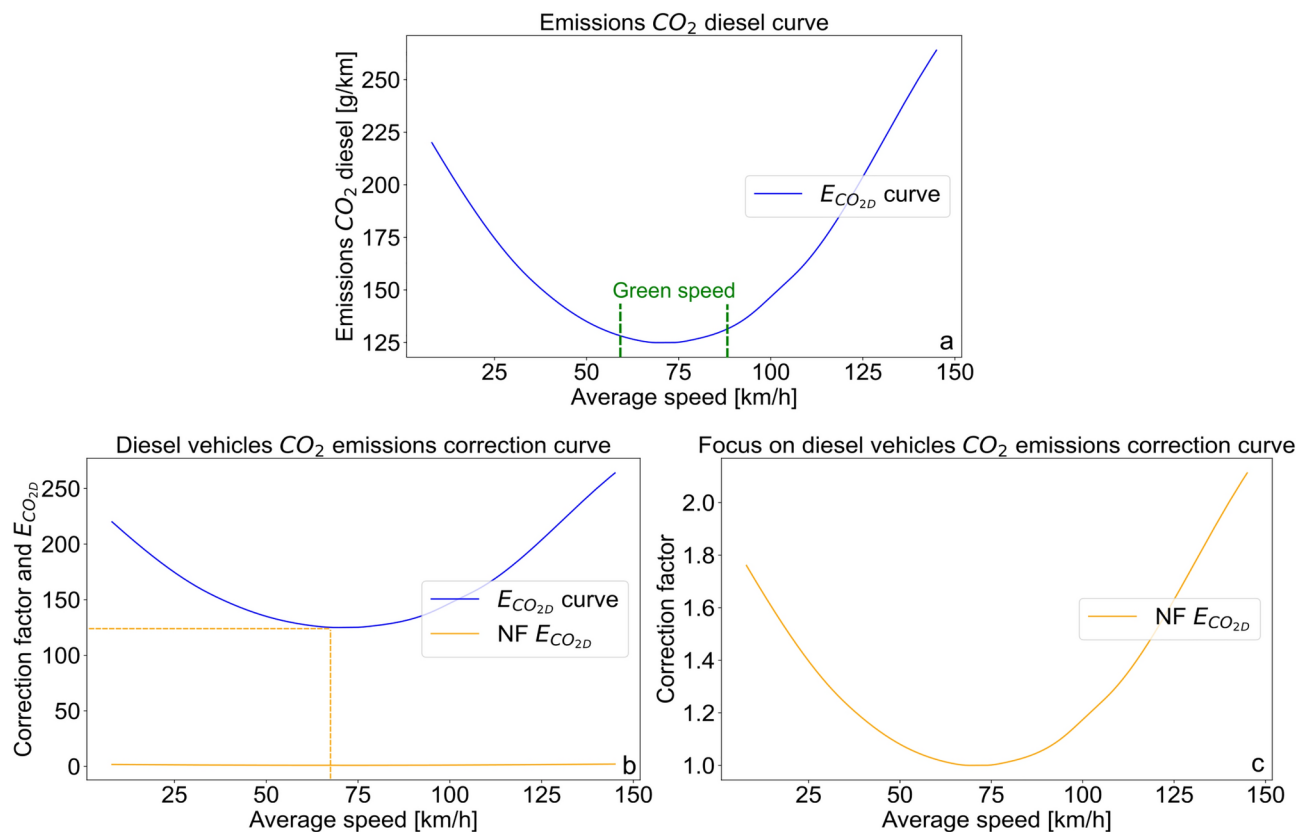
Fig. 2. a Mapping Average Speed vs. CO_2 emissions of Diesel Vehicles ( E_{CO_{2D}} ). b Normalized Emissions Curve ( NF E_{CO_{2D}} ) is obtained by normalizing the E_{CO_{2D}} curve against the minimum emissions value associated with speeds falling within the “Green Speed” range. This normalization is conducted under the assumption that the declared CO_2 emissions value provided by car manufacturers corresponds to this specific speed (69.28 km/h), with a reference value of 124.94 g/km. c A Close-up examination of the normalized emission curve for diesel vehicles.
